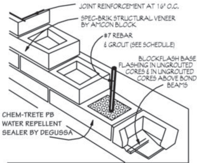
BASE FLASHING DETAIL
