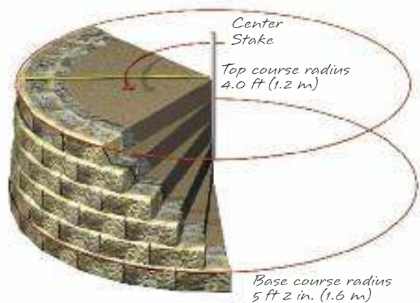
Base Course Radius for an outside curve on a 4 ft tall 6° wall
