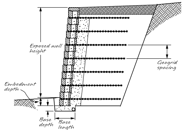
Typical Reinforcement Cross Section
