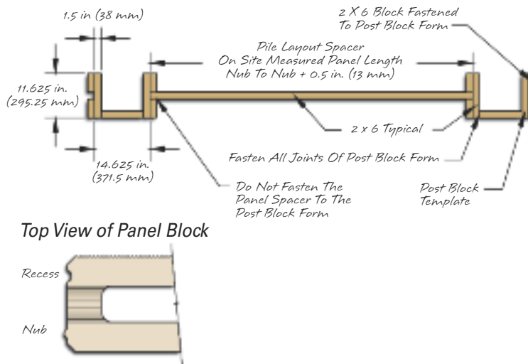
Figure 1: AB Fence Pile Layout Jig
