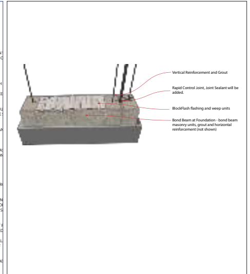
Figure 16a. Movement Joint
