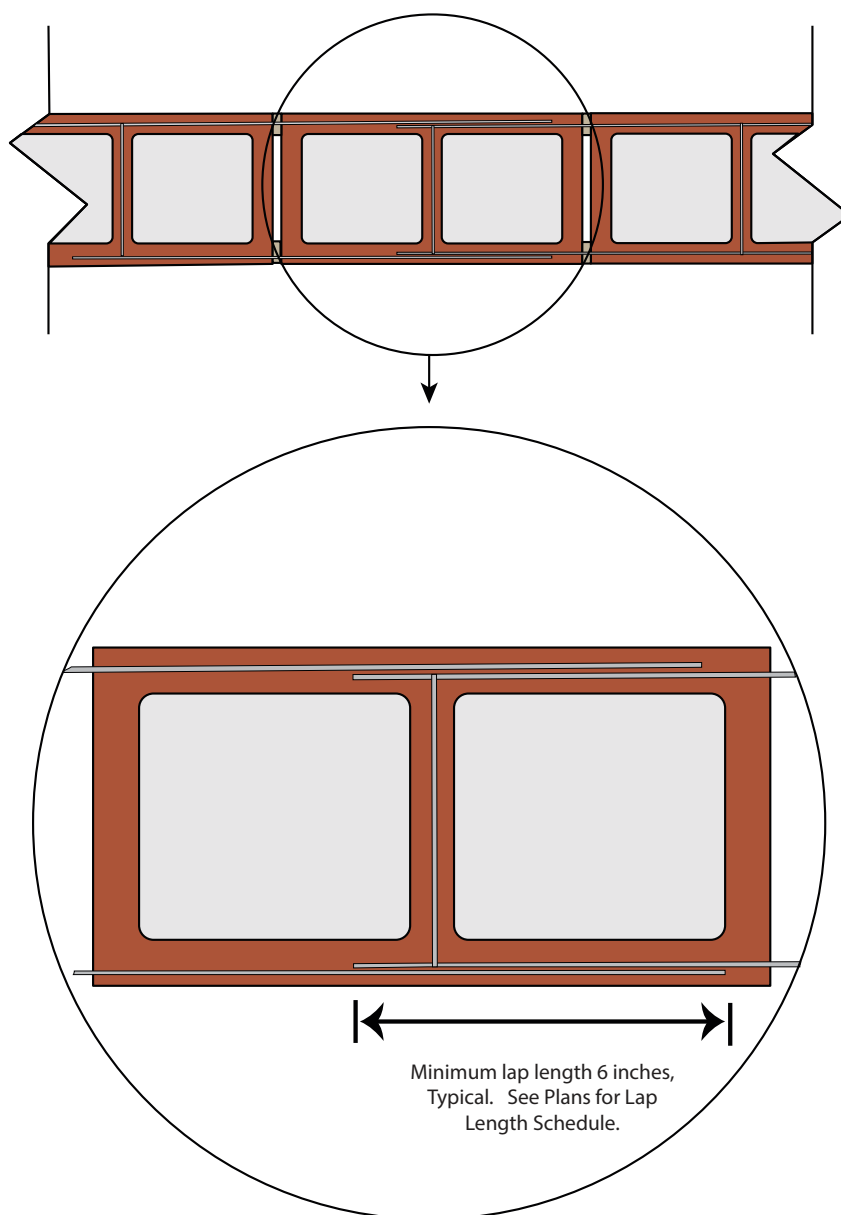
Figure 15. Joint Reinforcement
