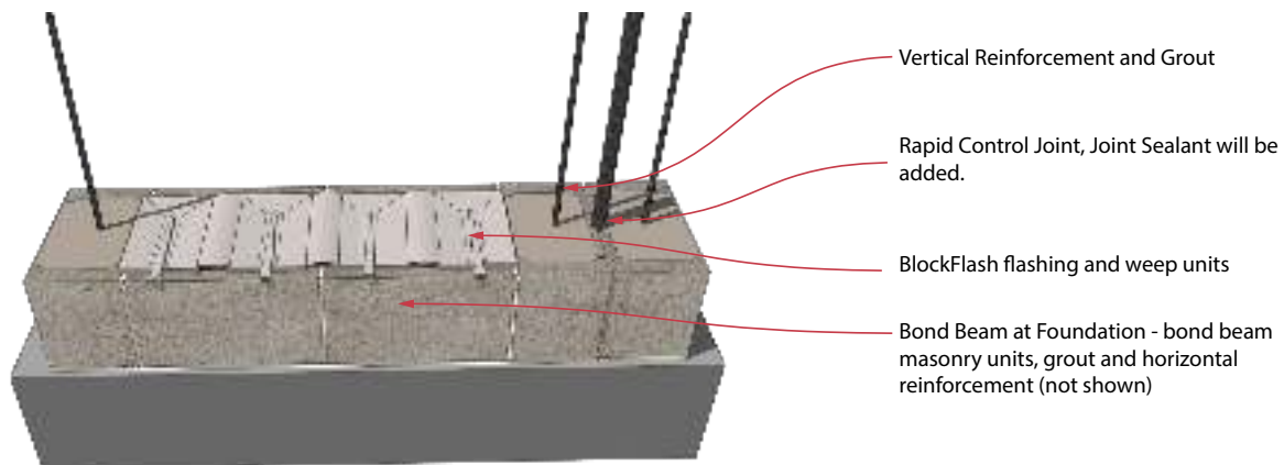
Sample Panel- Bond Beam Flashing Detail
