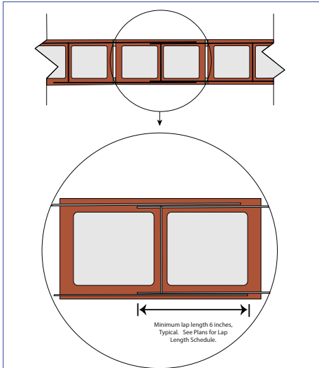
Figure 15. Joint Reinforcement
